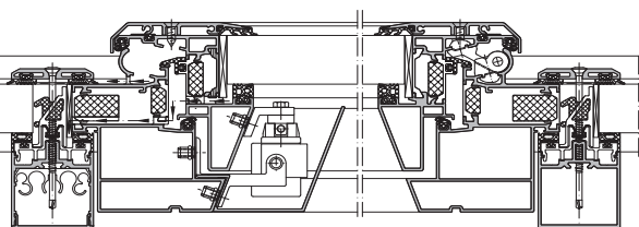
Schüco AWS 57 RO, lav karmprofil, M = 1:8
