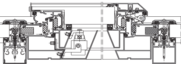
Schüco AWS 57 RO, "step"-glass, M = 1:8
